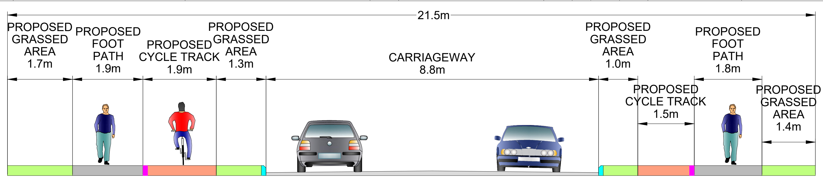
CROSS SECTION R-R
